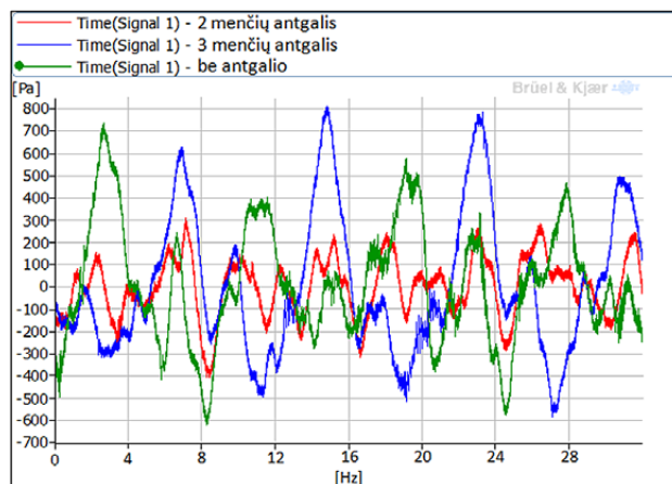
6 pav. Slėgio pokytis, kai giluminis kavitacinis aeratorius nuleidžiamas į vandens talpyklą \angle 50^\circ kampu Fig. 6. Difference in pressure when a deep-cavitation aerator is lowered \angle 50^\circ into a water tank
