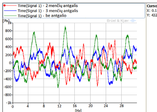
7 pav. Slėgio pokytis, kai giluminis kavitacinis aeratorius nuleidžiamas į vandens talpyklą \angle 30^\circ kampu Fig. 7. Difference in pressure when a deep-cavitation aerator is lowered \angle 30^\circ into a water tank
