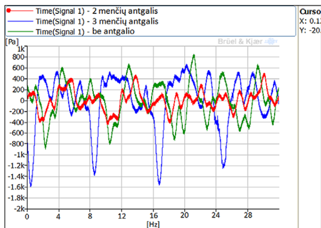
5 pav. Slėgio pokytis, kai giluminis kavitacinis aeratorius nuleidžiamas į vandens talpyklą \angle 65^\circ kampu Fig. 5. Difference in pressure when a deep-cavitation aerator is lowered \angle 65^\circ into a water tank
