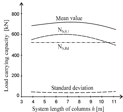
Fig. 14. Load carrying capacity for \bar{\lambda} = 1.0
