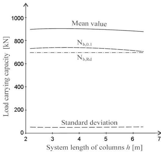
Fig. 10. Load carrying capacity for \bar{\lambda} = 0.6
