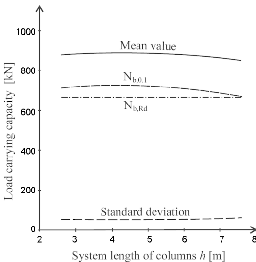
Fig. 11. Load carrying capacity for \bar{\lambda} = 0.7
